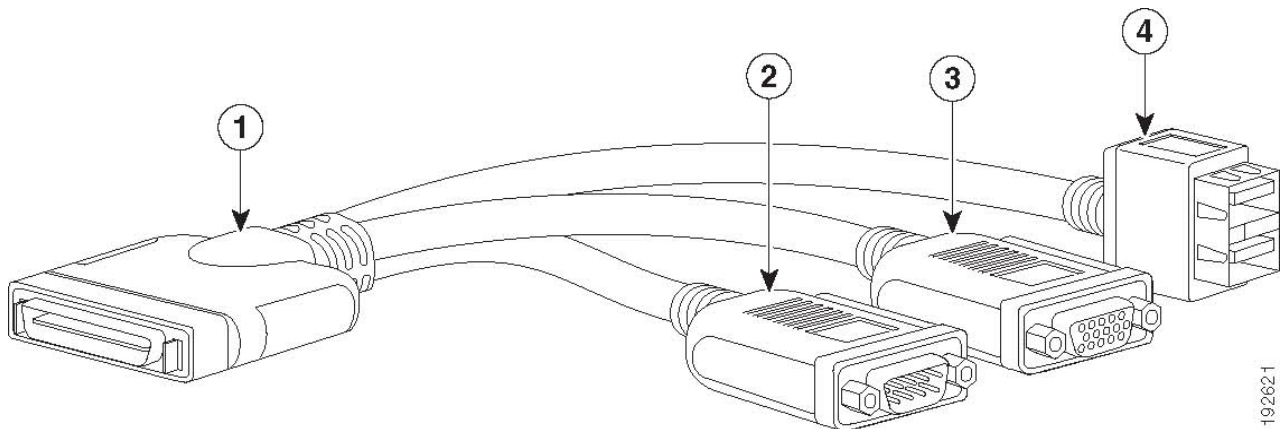
Figure 4 KVM Cable
