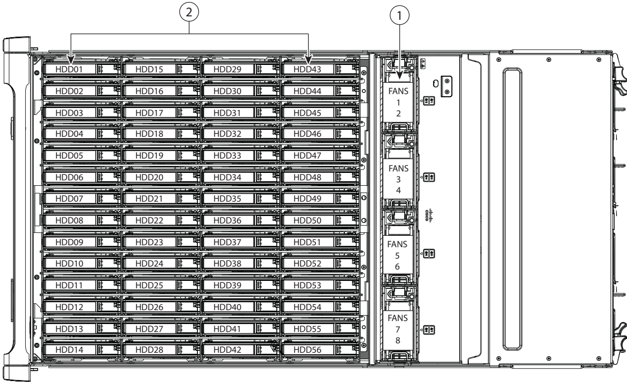
Figure 5 C3160 Server With Top Cover Off
