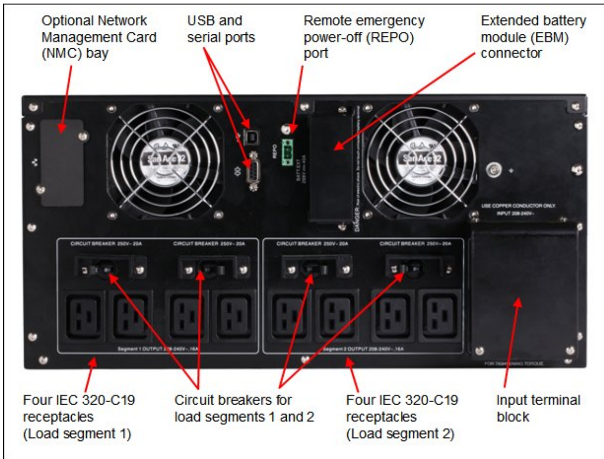
Figure 3. Rear panel of the IBM 11000VA LCD 5U Rack UPS
