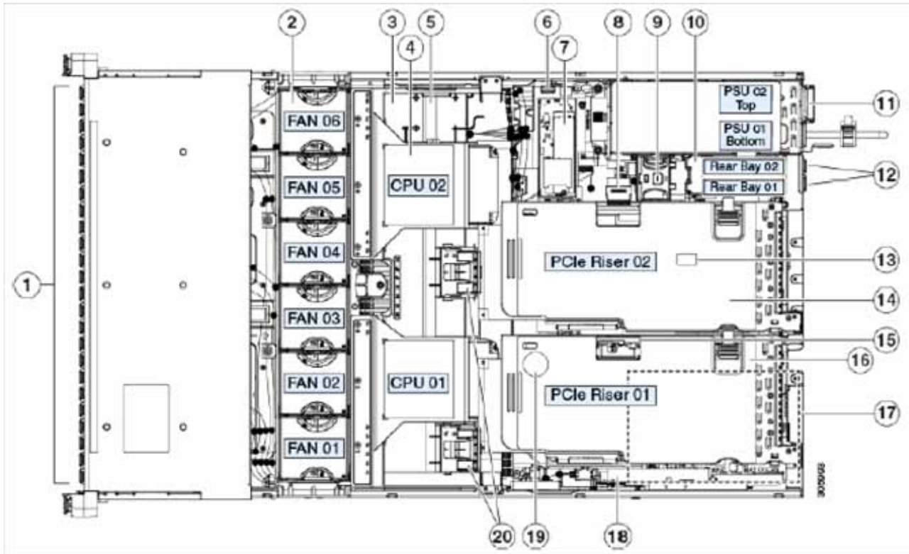
Figure 6 C240 M5 SFF With Top Cover Off
