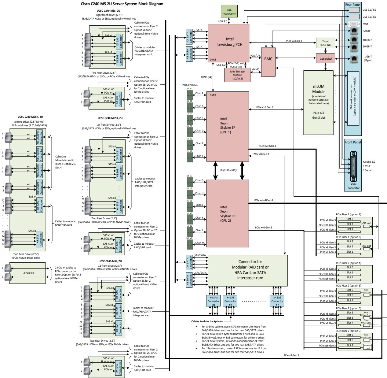
Figure 7 C240 M5 Block Diagram
