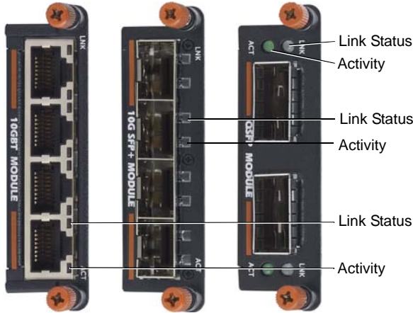
Figure 1-6. Port LEDs on Modules
