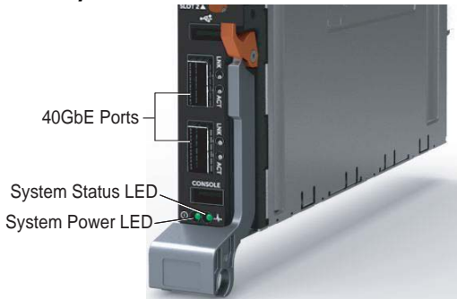
Figure 1-5. System LEDs on Front Panel
