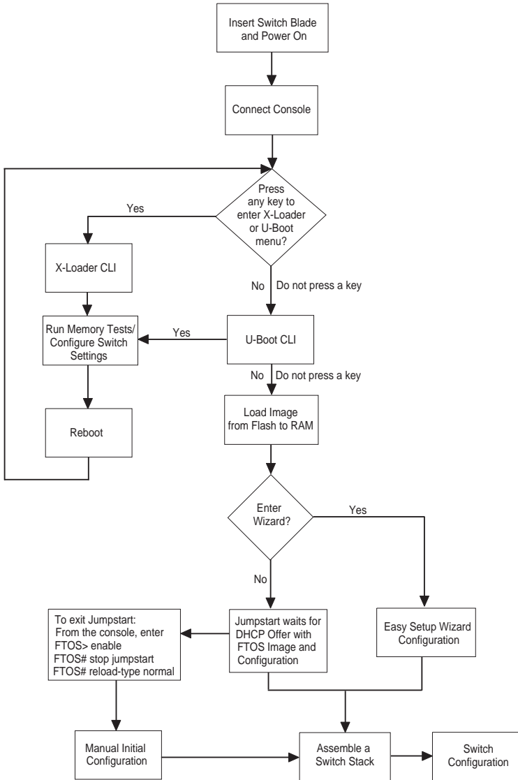
Figure 1-7. MXL 10/40GbE Switch: Installation and Configuration Flow Chart
