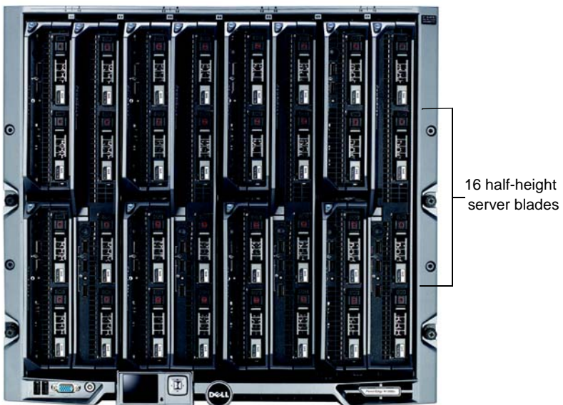
Figure 1-8. PowerEdge M1000e: Front View with Server Blades
